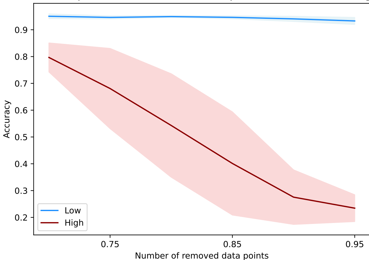
DataAttrOpt(5000, 0.03, 15, best, +b, alpha=best) - bbc-embeddings
